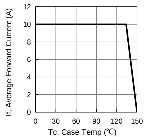
Current derating curve, per element
